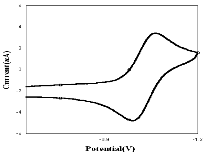
Figure 1. Cyclic voltammogram of 1 mM [Et 4 N][V(CO) 4 (dppe)] in acetonitrile/0.1 M n -Bu 4 NPF 6 with a scan rate of 50 mV/s.
